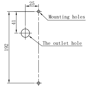
Mounting holes
