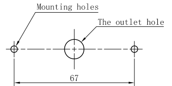
Mounting holes
