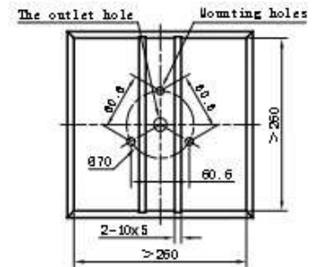
Mounting holes
