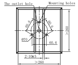
Mounting holes
