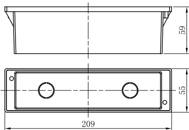
Recessed Box
