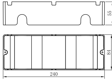
Recessed Box
