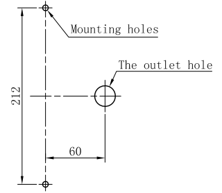
Mounting holes
